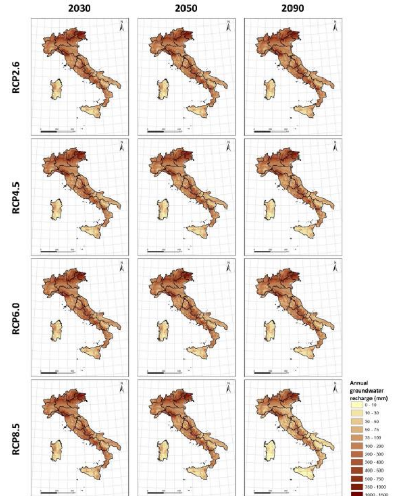
Fig. 8 Projections of 20-year average of annual groundwater recharge (mm) for four emission scenarios (rows) and three time horizons (columns)
