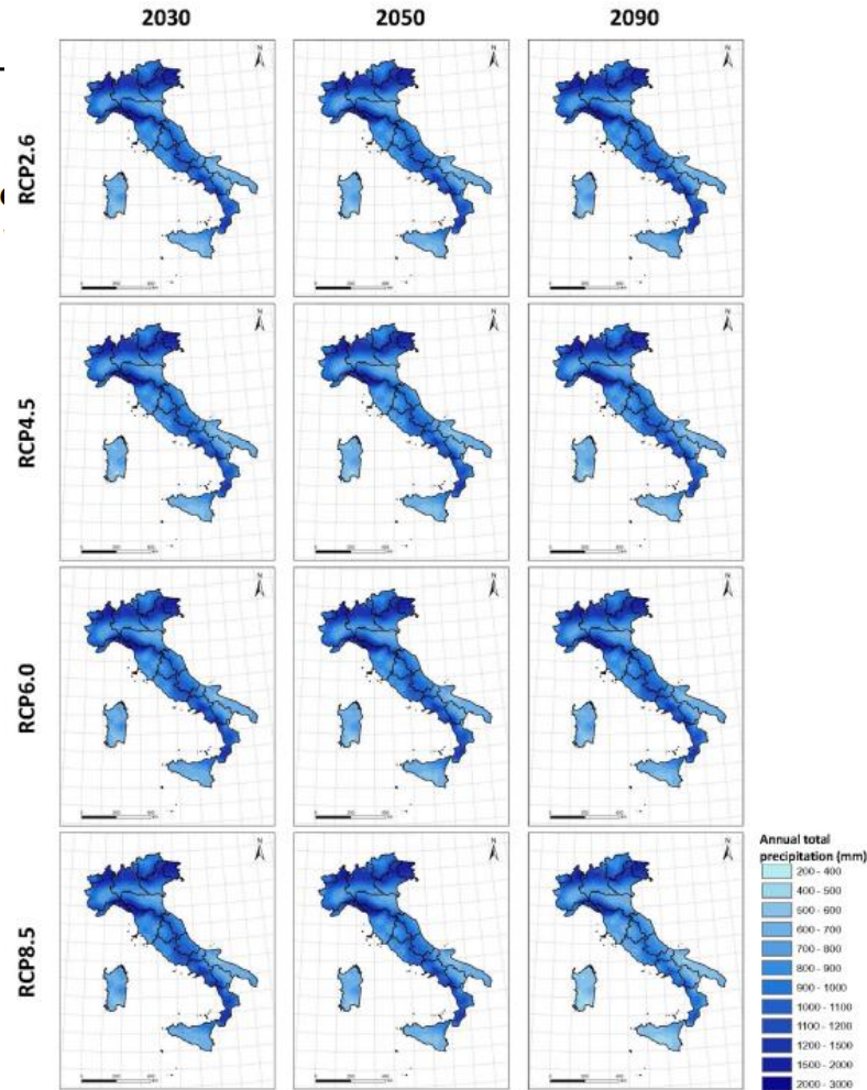
Fig. 6 Projections of 20-year average of annual total precipitation (mm) for four emission scenarios (rows) and three time horizons (columns)
