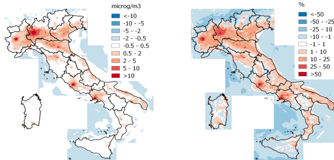
Differenza assoluta ( \mu\text{g}/\text{m}^3 )
